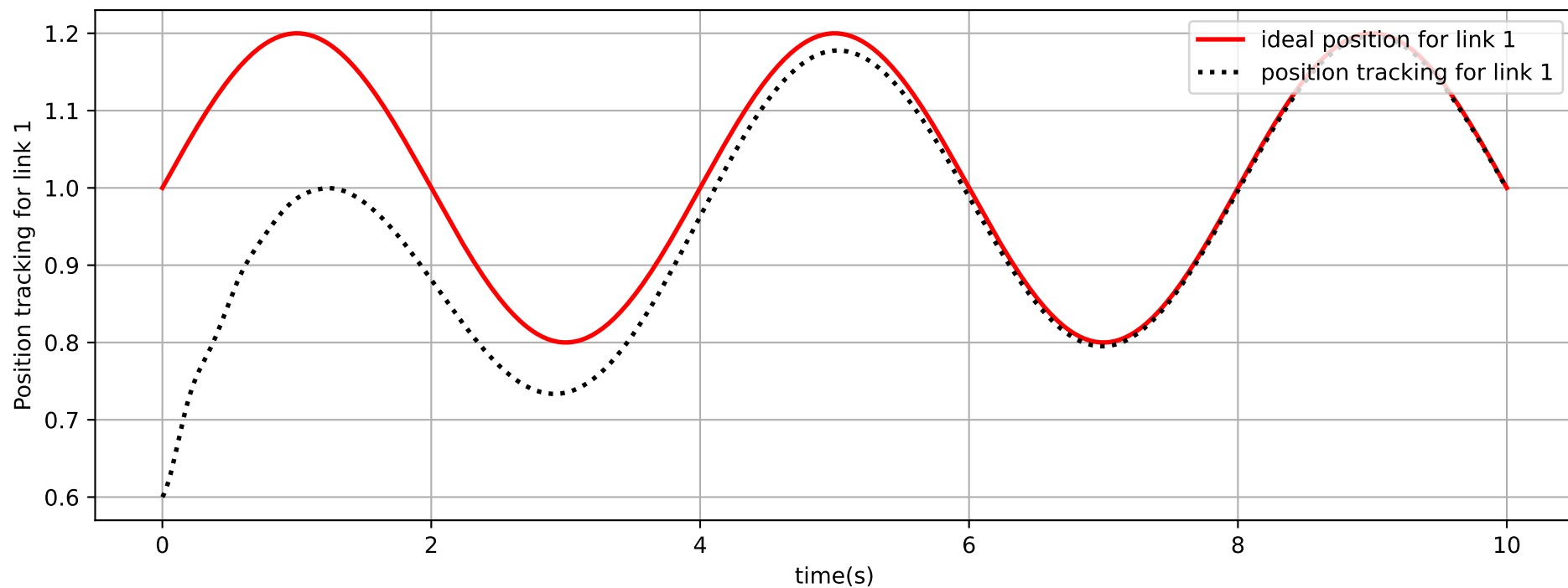
Position Tracking Performance ( S=3 , S1=1 , m=5 )
